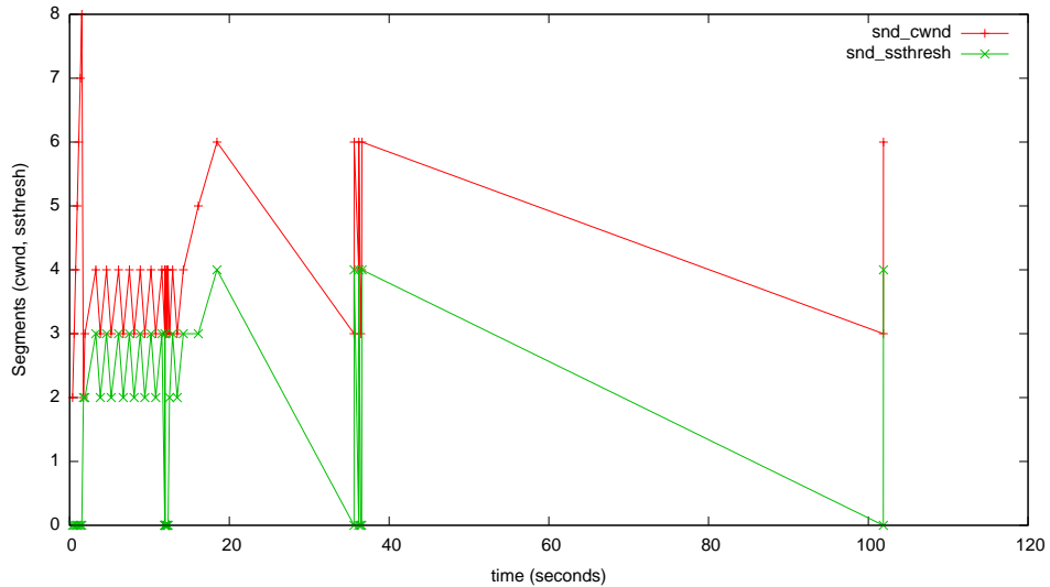
myTcpProbeData - vegas-mode=1
