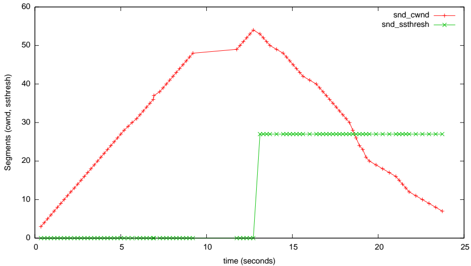
myTcpProbeData - westwood-mode=1
