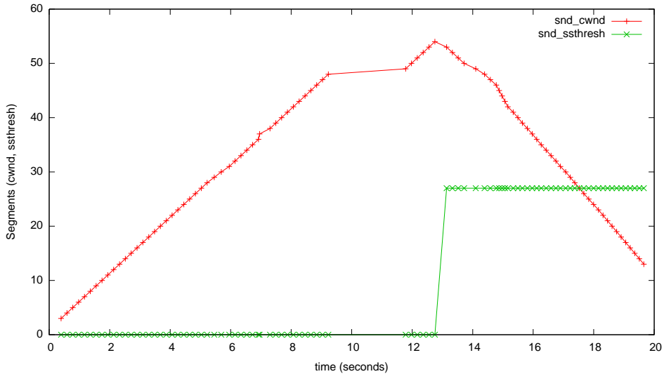
myTcpProbeData - westwood-mode=2
