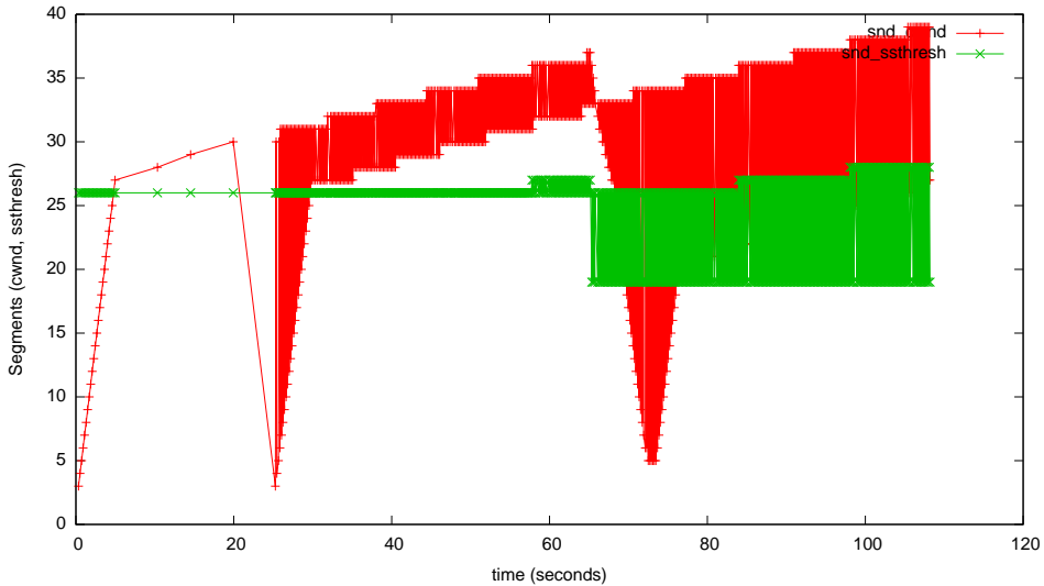
myTcpProbeData - yeah-mode=3
